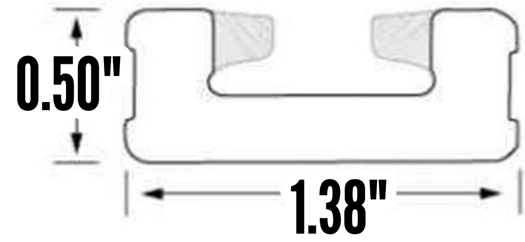
PROFILE VIEW:
