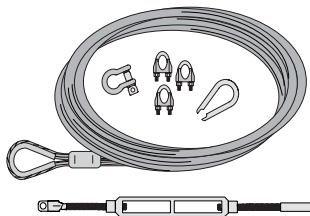
3/8 in cable with termination hardware and turnbuckle
