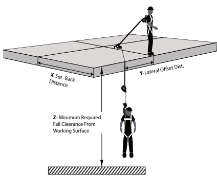
Figure 12 - FT-X Minimum Required Fall Clearance for 130 to 310 lbs. (59 to 141 kg) Users
