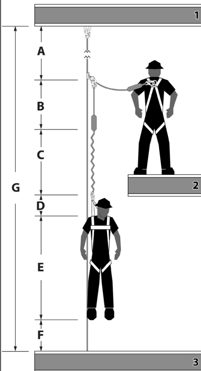
Figure 6 - Managing Stretch Minimum Clear Fall Requirement: Vertical Lifeline System
