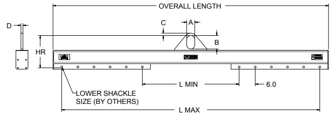
LIFTING BEAM - LOW HEADROOM ADJUSTABLE
