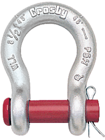
G-213/S-213 G-213 Round pin anchor shackles meet the performance requirements of Federal Specification RR-C-271F Type IVA, Grade A, Class 1, except for those provisions required of the contractor. For additional information, see page 452.
